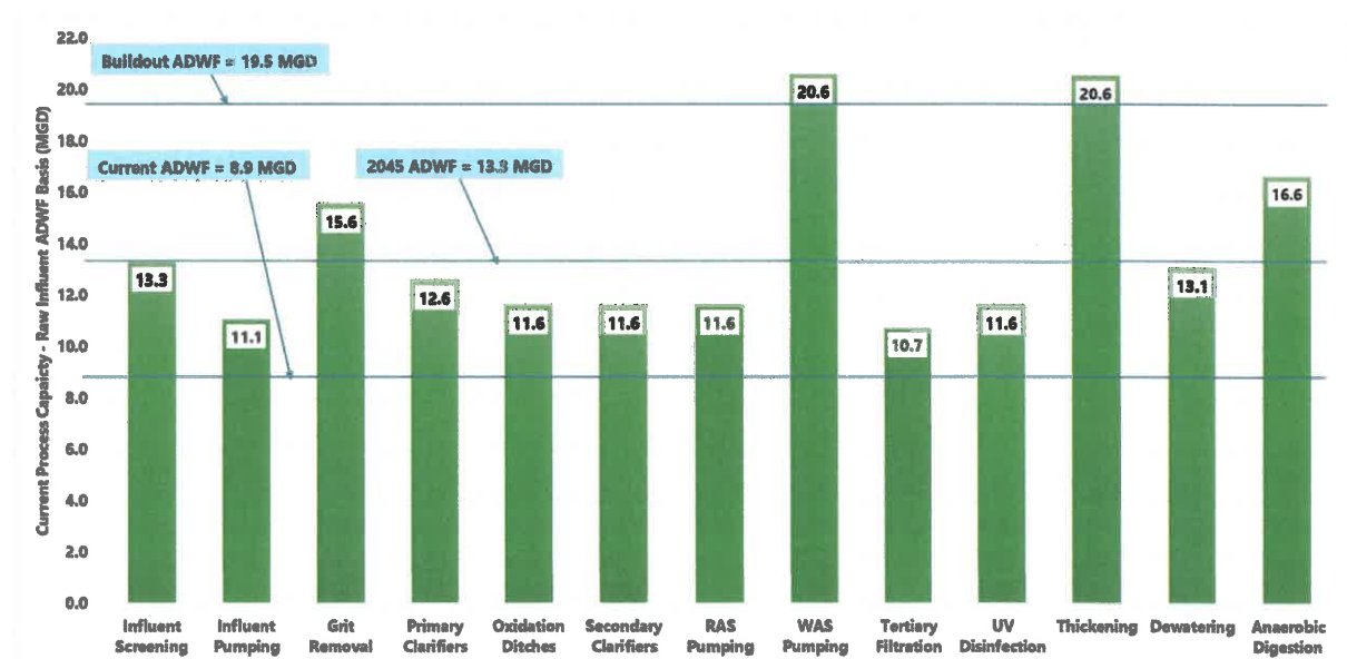
FIGURE ES-2: PGWWTP CURRENT PROCESS CAPACITY UTILIZATION
