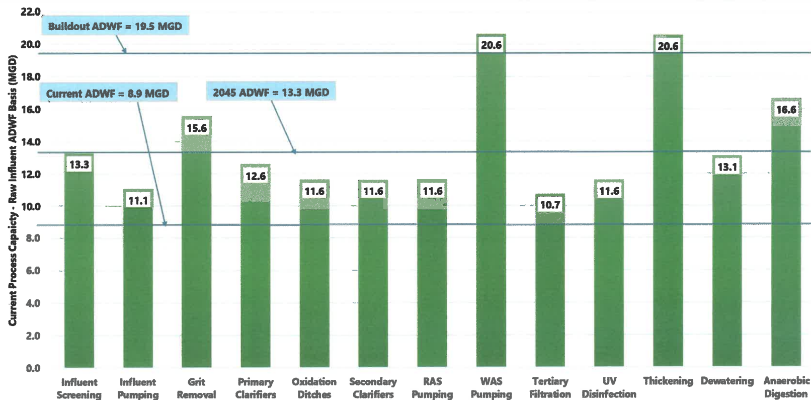
FIGURE 3-1: PGWWTP CURRENT PROCESS CAPACITY UTILIZATION
